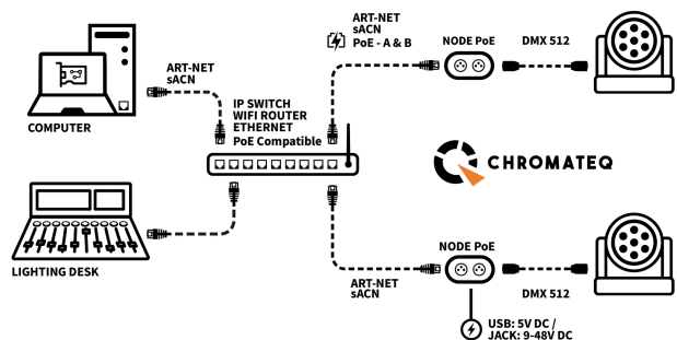
NODE mode, Art-Net / sACN network
